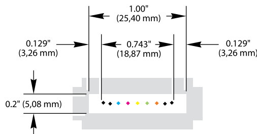
White Space Requirements for 6-color Lateral Marks
