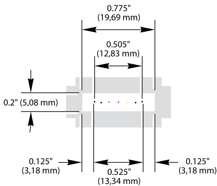
White Space Requirements for 4-color Lateral Marks
