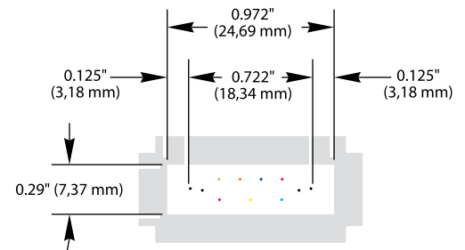
White Space Requirements for 8-color Lateral Marks
