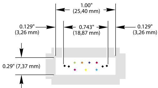
White Space Requirements for 8-color Lateral Marks
